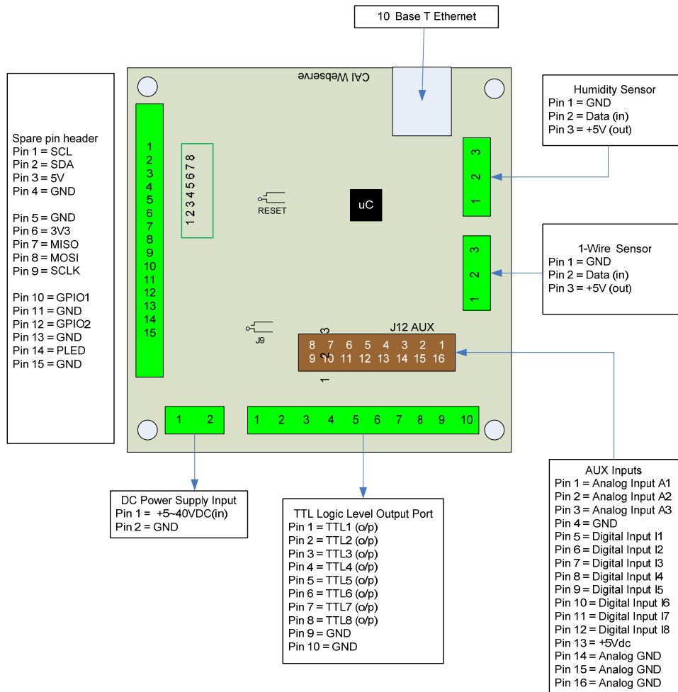
Figure 1.0 WebControl™ PCB inputs and outputs diagram
